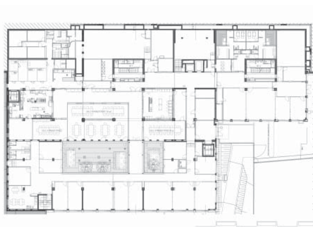
Plan level 8
