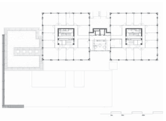
Plan level 10
