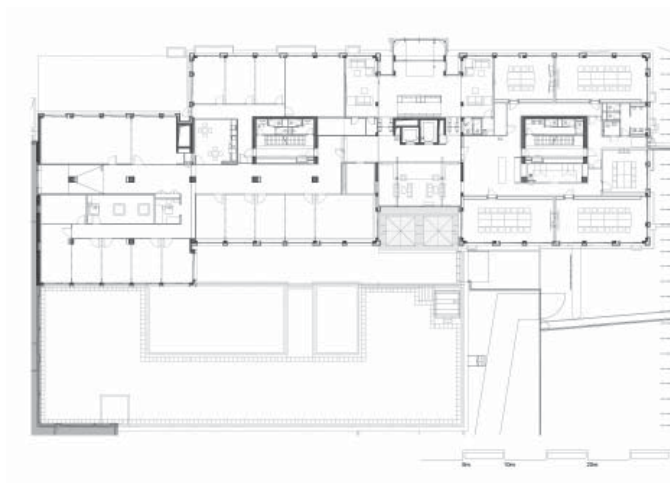
Plan level 9
